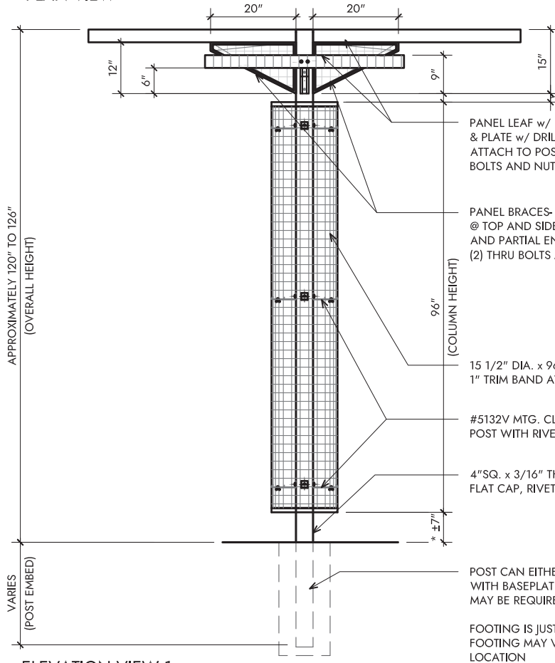
ELEVATION VIEW 1
