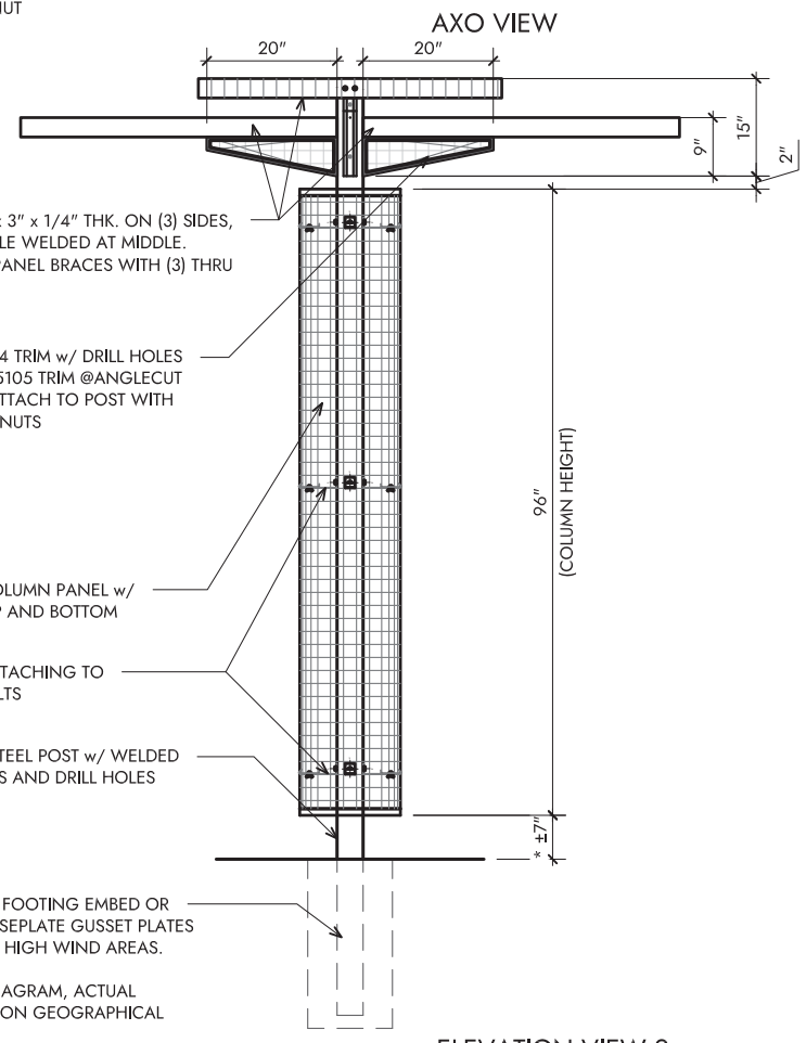
ELEVATION VIEW 2
